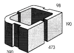
20.57 PIASTER WITH CONTROL JOINT
