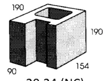
20.24 (NC) JAMB-HALF
