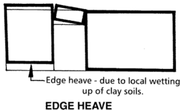
Figure 22 Consequences of distortions of supports of walls with openings
