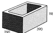
30.925 SINGLE CORE
