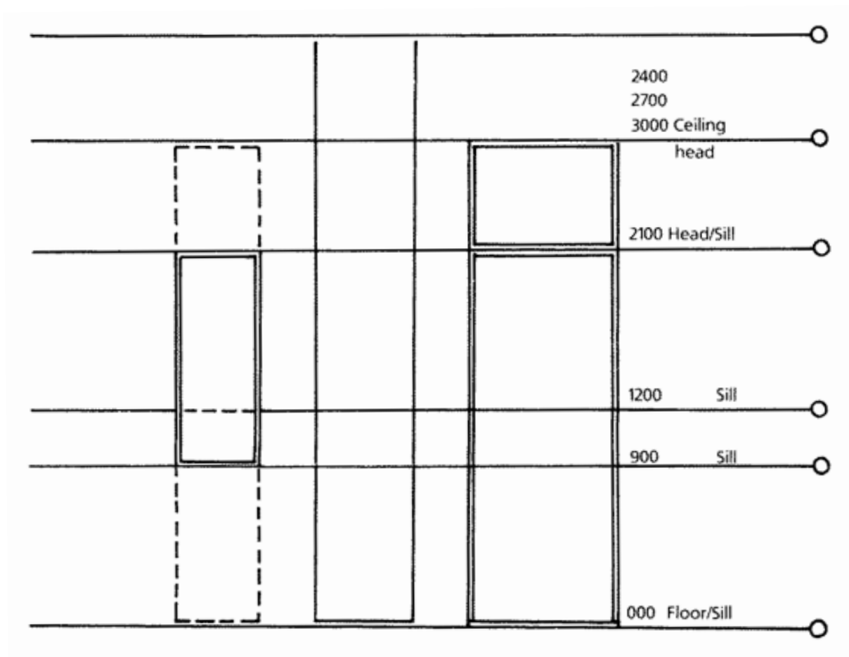
Figure 14 Vertical modular dimensions
