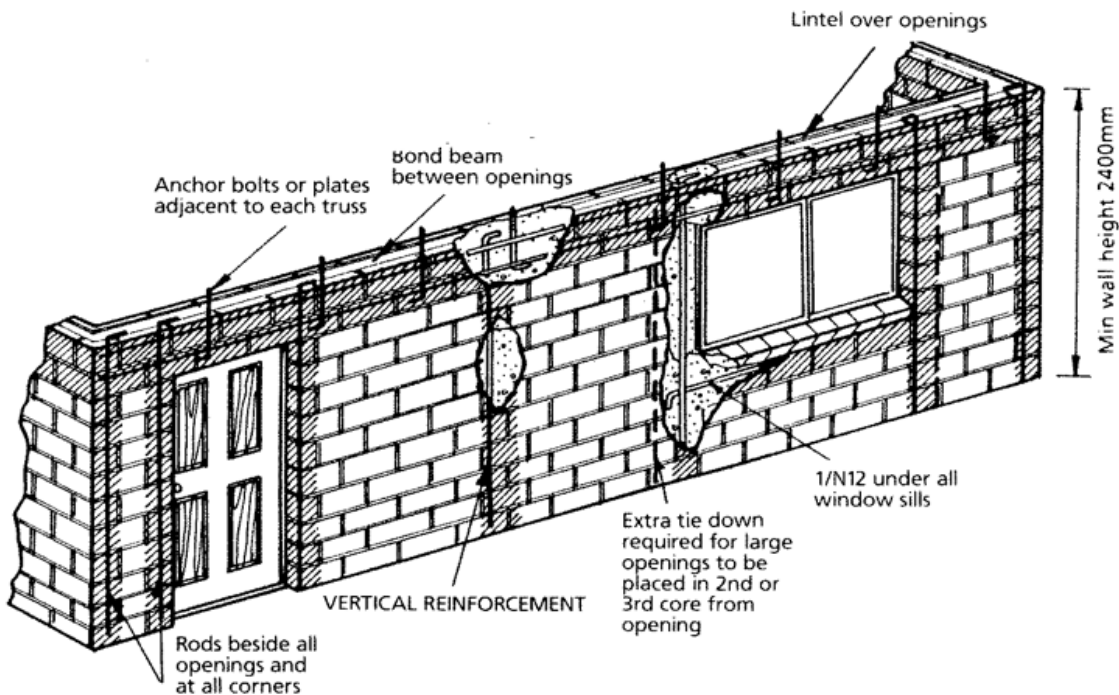
Figure 28 Typical construction details for reinforced single-leaf masonry walling system
