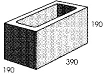
20.925 SINGLE CORE
