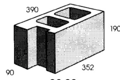
20.23 JAMB-FULL LENGTH
