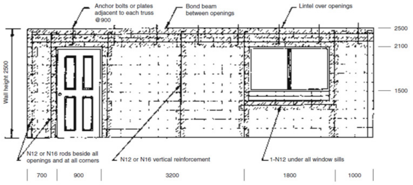
Figure 36 Typical single-leaf masonry details
