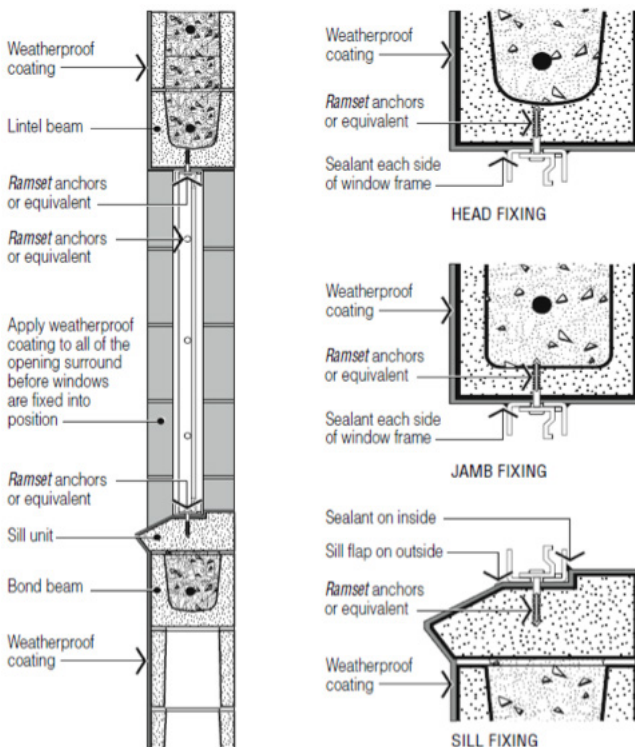
Figure 26 Weatherproofing and fixing of windows in single-skin masonry construction
