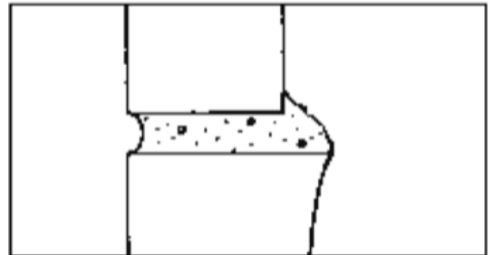
Figure 6 Ironed finish (face-shell cross section)
