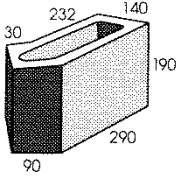
15.739 45° SQUINT
