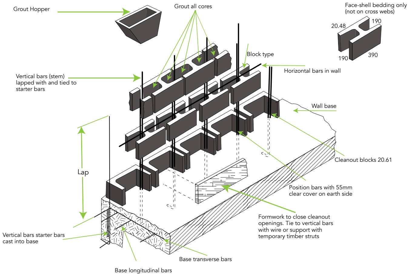
Figure 27 Typical construction details for reinforced blockwork retaining wall
