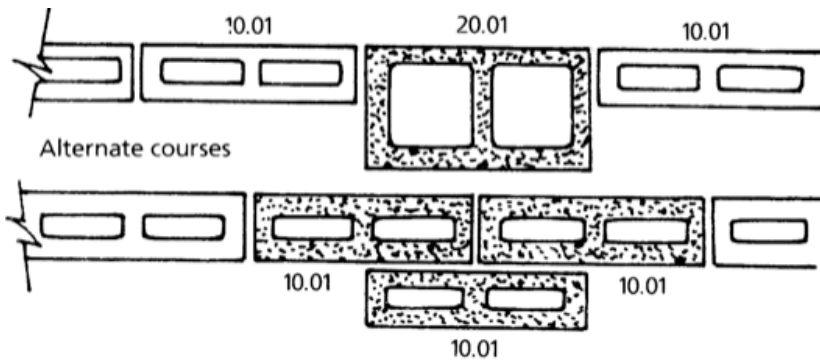
Figure 13 Engaged pier in 100 mm hollow-block wall
