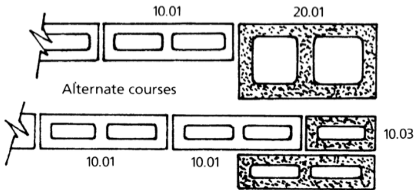
Figure 12 Pier at end of 100 mm hollow-block wall
