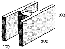
20.48 "H" BLOCK
