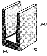
20.18 DEEP LINTEL
