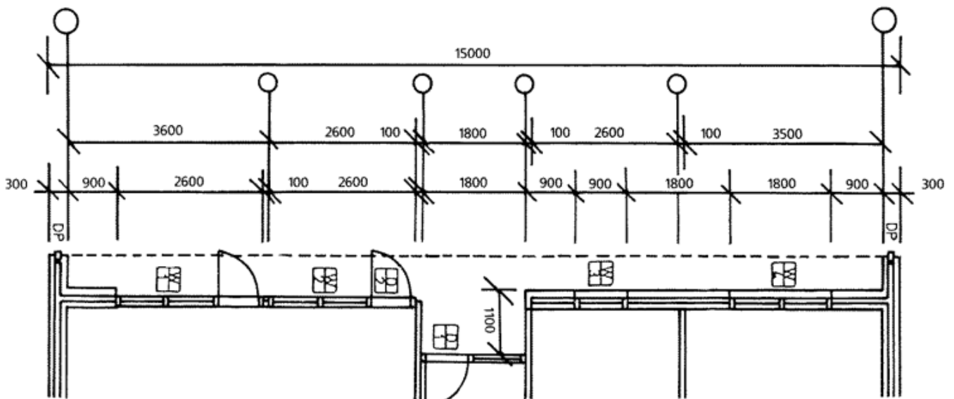
Figure 15 Preferred method of dimensioning drawings using the nominal sizes of openings
