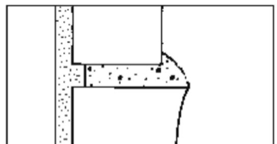
Figure 8 Raked finish with render
