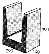
30.18 DEEP LINTEL
