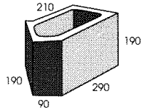
20.739 45° SQUINT
