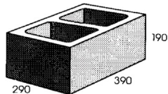
30.01 STANDARD
