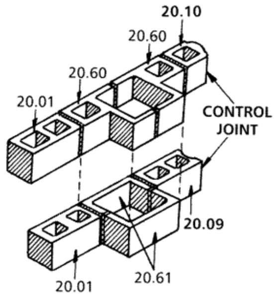
Figure 19 Typical control joint within a wall
