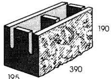
20.120 KNOCK-OUT BOND BEAM
