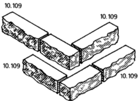
Figure 10 Typical split-block corner details
