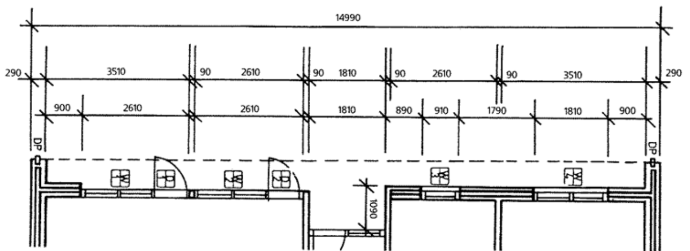
Figure 16 The equivalent actual size of openings
