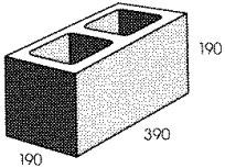
20.01 STANDARD
