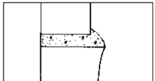
Figure 7 Flush finish (face-shell cross section)
