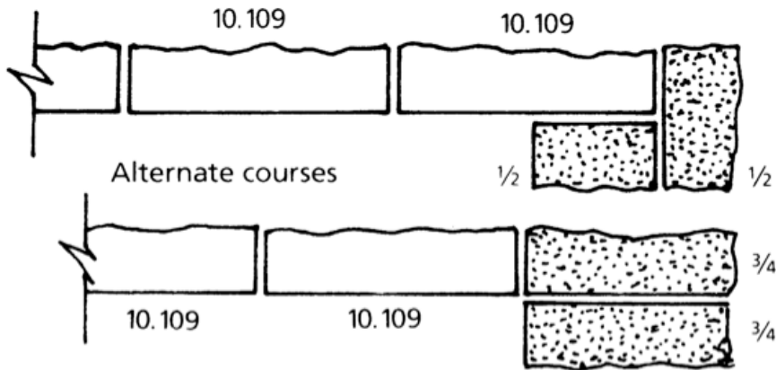
Figure 11 Pier at end of 100 mm split-block wall
