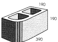
20.713 BULLNOSE
