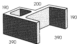
20.60 BONDED PIER
