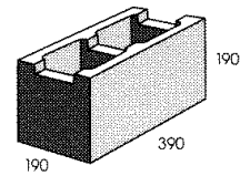
20.42 CHANNEL
