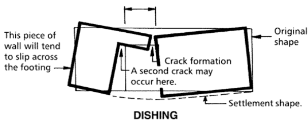
Figure 24 Behaviour of articulated wall after distortion of supporting members
