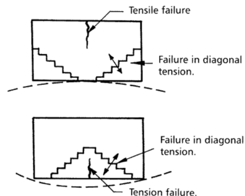
Figure 17 Differential settlement of footings
