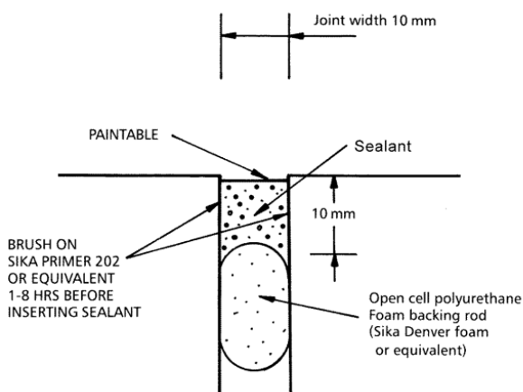
Figure 25 Control joint detail
