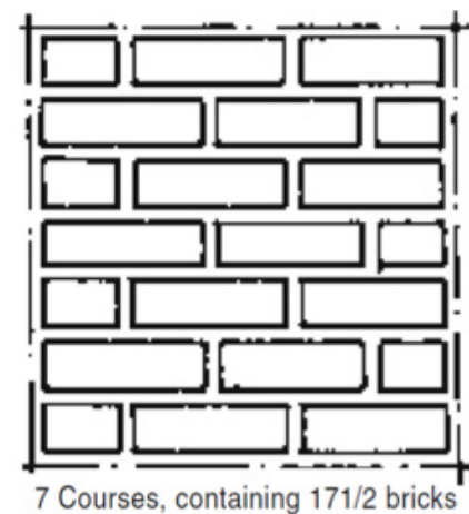
Figure 1 Number of blocks and bricks in a 600-mm building module
