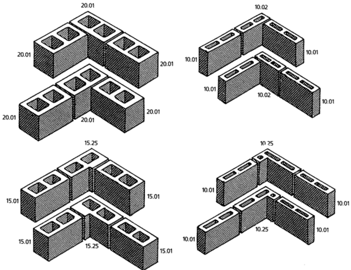
Figure 9 Typical hollow-block corner details
